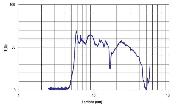
Graphic 2: Transmission of the silicon window.
